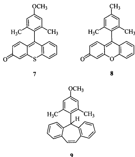
Scheme 3. Additional isolated and identified products.
