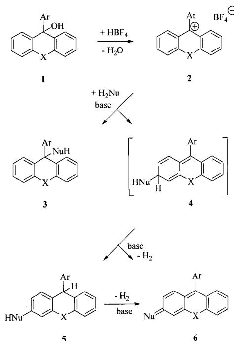
Scheme 1. Mechanistic rationale for the reactions of nucleophiles with triarylmethyl salts of type 2 .
