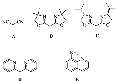
Scheme 2. List of the tested C- and N-nucleophiles (or pre-nucleophiles, respectively).
