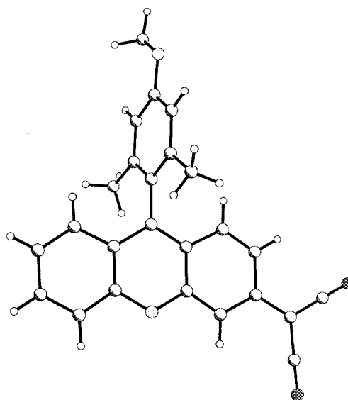
Figure 1. Structure of p -quinoid dibenzopyran 6.2A in the crystal. [9]
